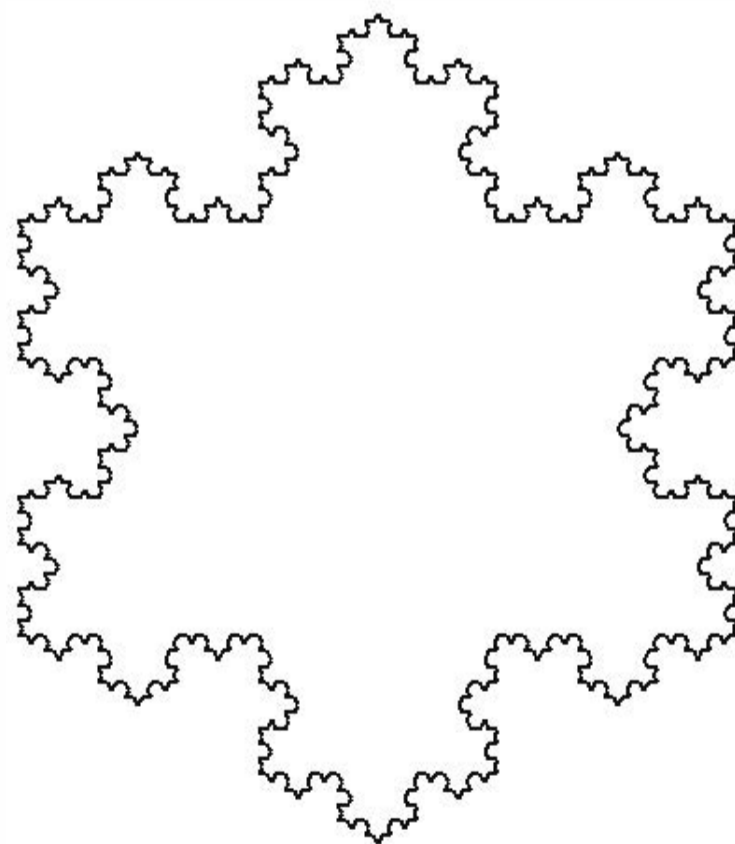
Figure 13.7: Koch snowflake
